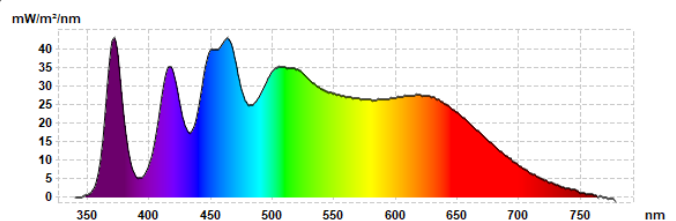
Spectrum DLS Color Proof Light D65
